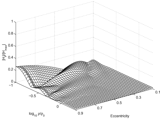
Fig. 7 Fractional momentum remaining using the affine partial-state controller.
