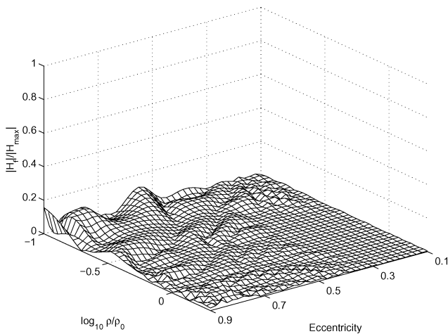
Fig. 8 Fractional momentum remaining using the two-stage controller.
