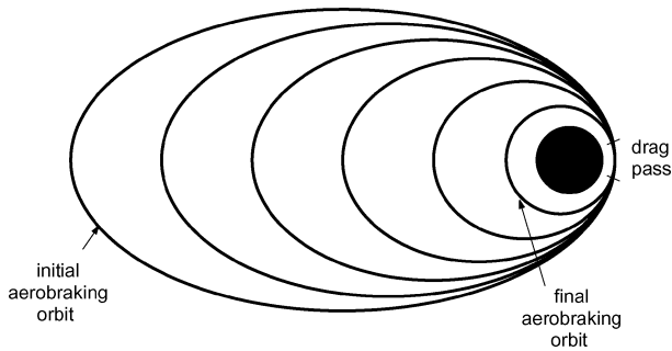
Fig. 2 Orbit decay using aerobraking.
