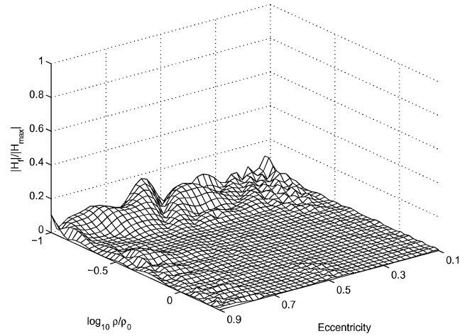
Fig. 5 Fractional momentum remaining using the two-stage controller.
