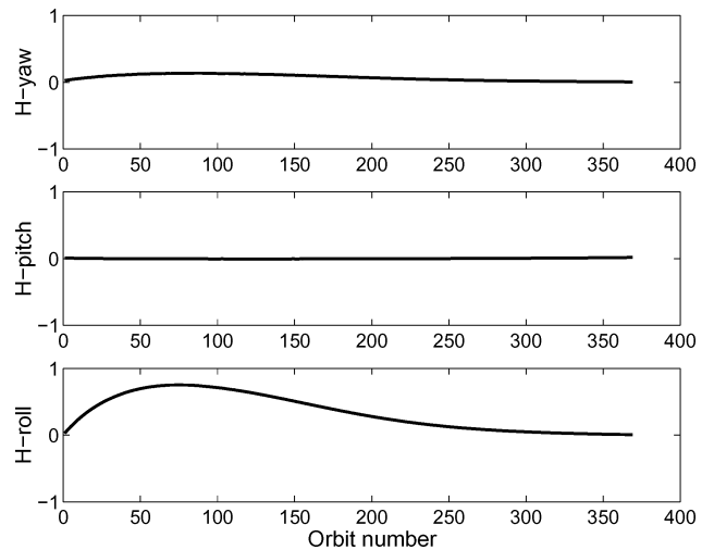
Fig. 10 Momentum of the spacecraft after each drag pass using the affine partial-state controller.
