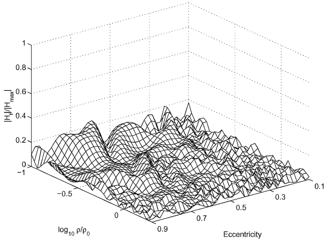
Fig. 3 Fractional momentum remaining after a drag pass for the spin-down controller where the independent variables are relative density and eccentricity.
