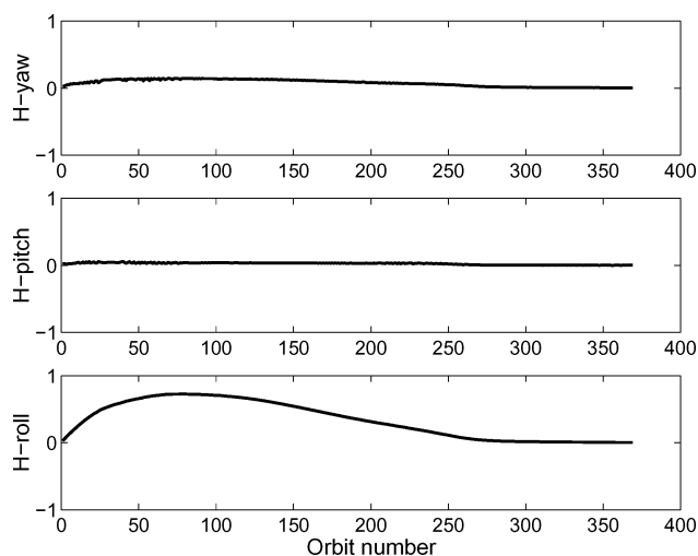
Fig. 11 Momentum of the spacecraft after each drag pass using the two-stage controller.
