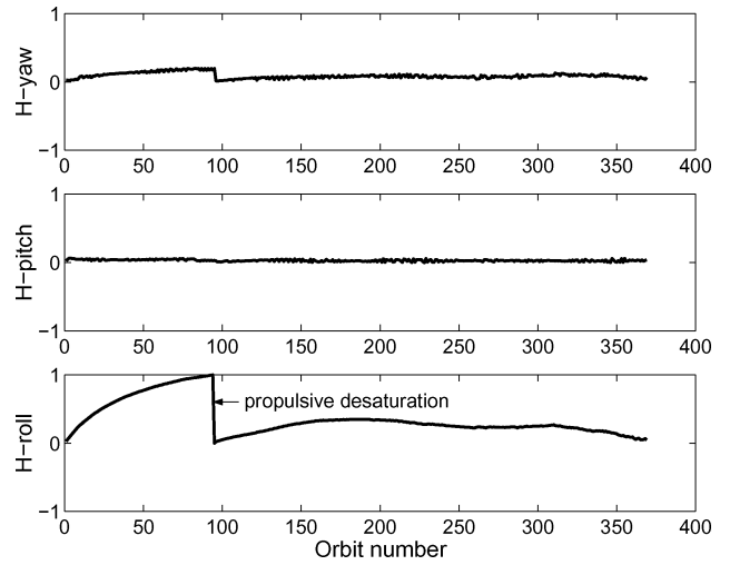
Fig. 9 Momentum of the spacecraft after each drag pass using the spin-down controller with an initial orbit period of 48 h and a final orbit period of 2 h.
