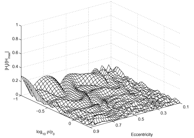
Fig. 6 Fractional momentum remaining using the spin-down controller where initial stored momentum is along the pitch (+Y) axis at 27 kg · m 2 /s (100% capacity).
