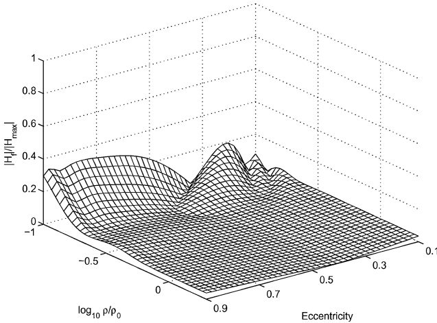
Fig. 4 Fractional momentum remaining using the affine partial-state controller.
